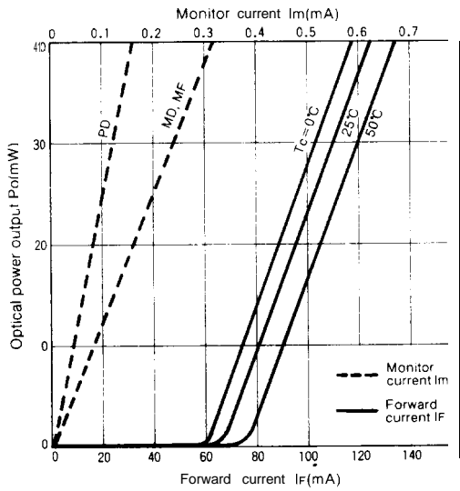
Fig. 81-3 Threshold Current vs. Temperature
