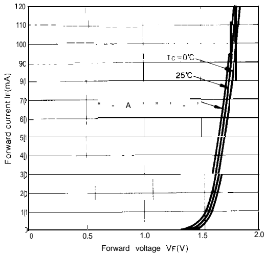
Fig. 81-1 Forward Current vs. Forward Voltage
