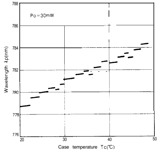
Fig. 81-4 Wavelength vs. Temperature
