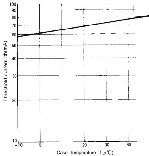
Fig. 81-3 Threshold Current vs. Temperature
